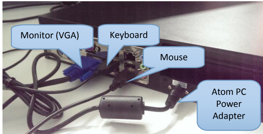
Figure 1 Atom PC (Rear view)
